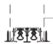
SDS Type 8A Concealed Plaster Frame Screw Mounting
