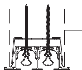
SDS Type 2 Flange Frame Concealed Mounting
