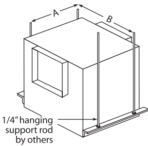
CK Hanging Vibration Isolators
