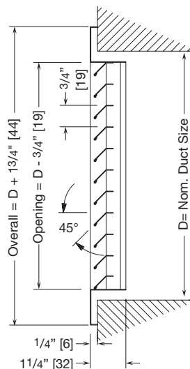
3/4" (19) Blade Spacing Fixed Louvers, No Damper
